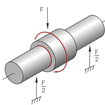
Fig. 10: Rotating load, shaft stationary, bush rotating
